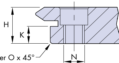
Tapped Hole Option N
