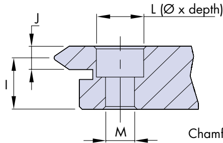
Standard Counterbored Hole
