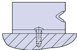
Blind Fixing Flanged Type
